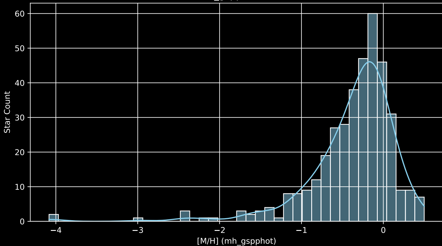
APOGEE DR17 Field: [ORIONB-B [M/H] (mh_gspphot) (n= 379)
