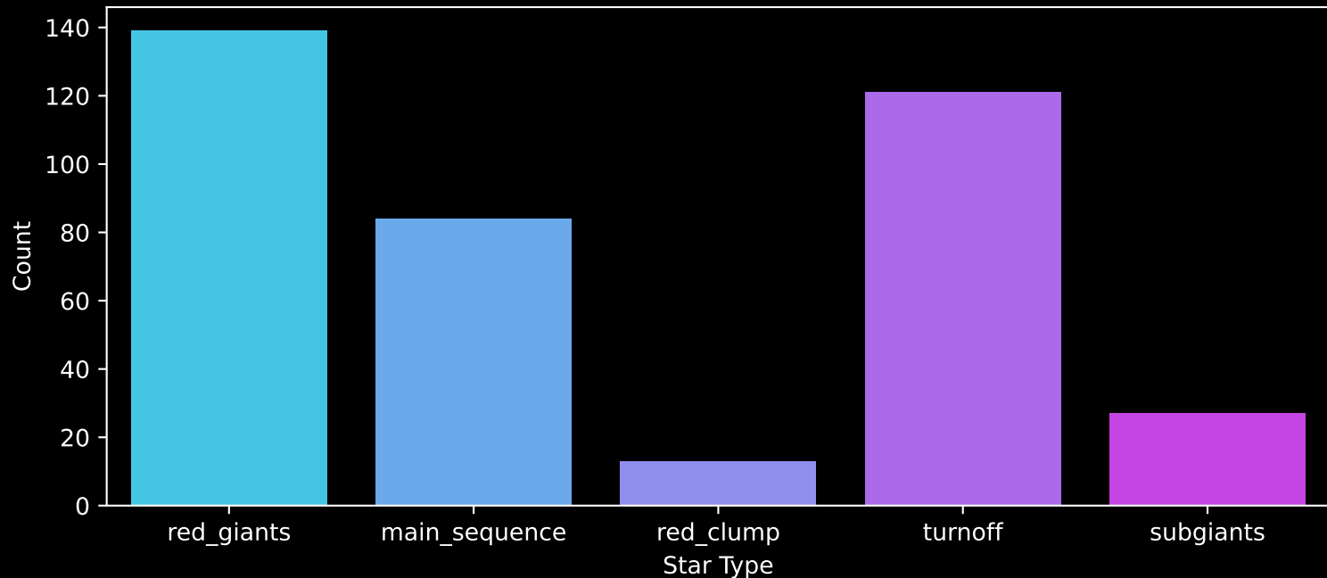
APOGEE DR17 Field: [ORIONB-B] Count plot of Star Type
