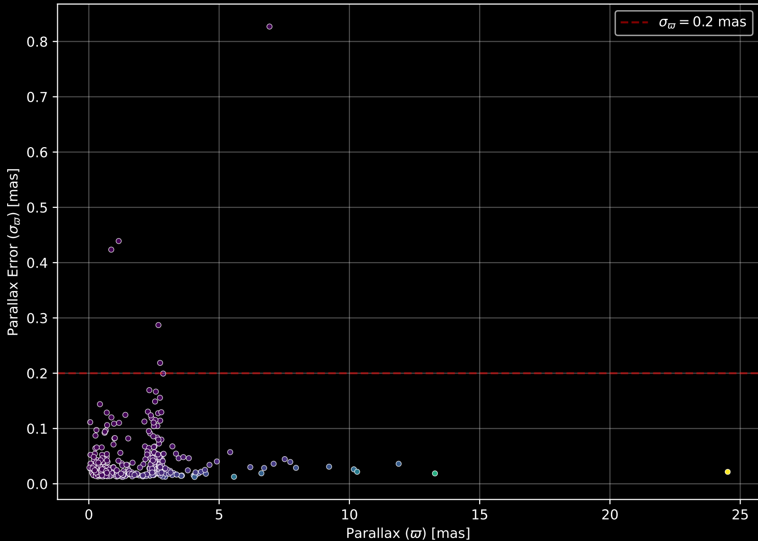
APOGEE DR17 Field: [ORIONB-B] Parallax Quality (n= 384)
