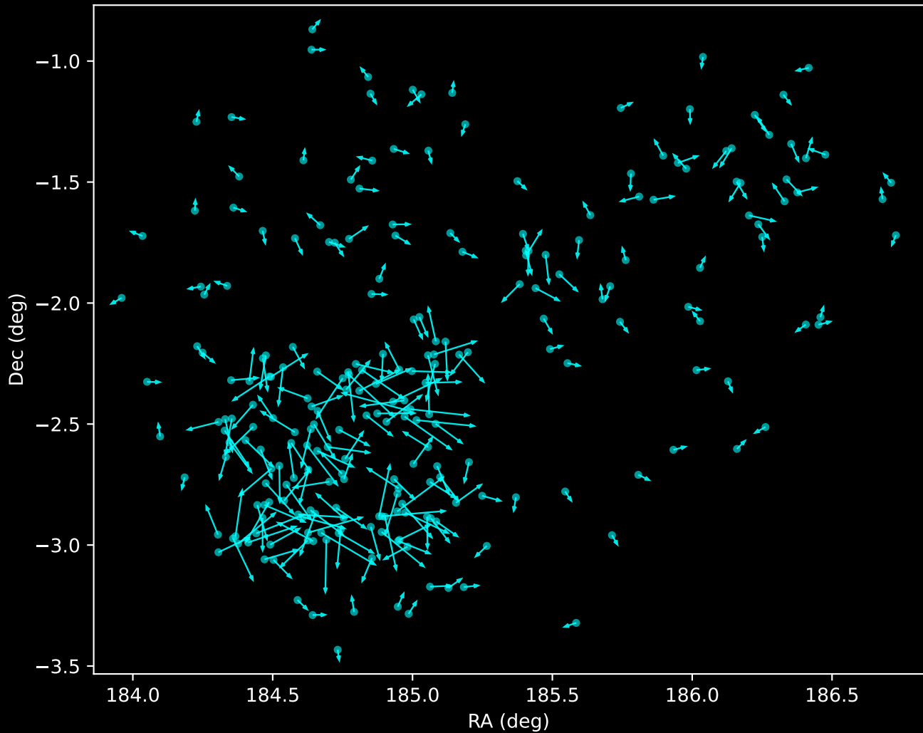
APOGEE DR17 Noise Stream Proper Motion Vectors (n=241)
