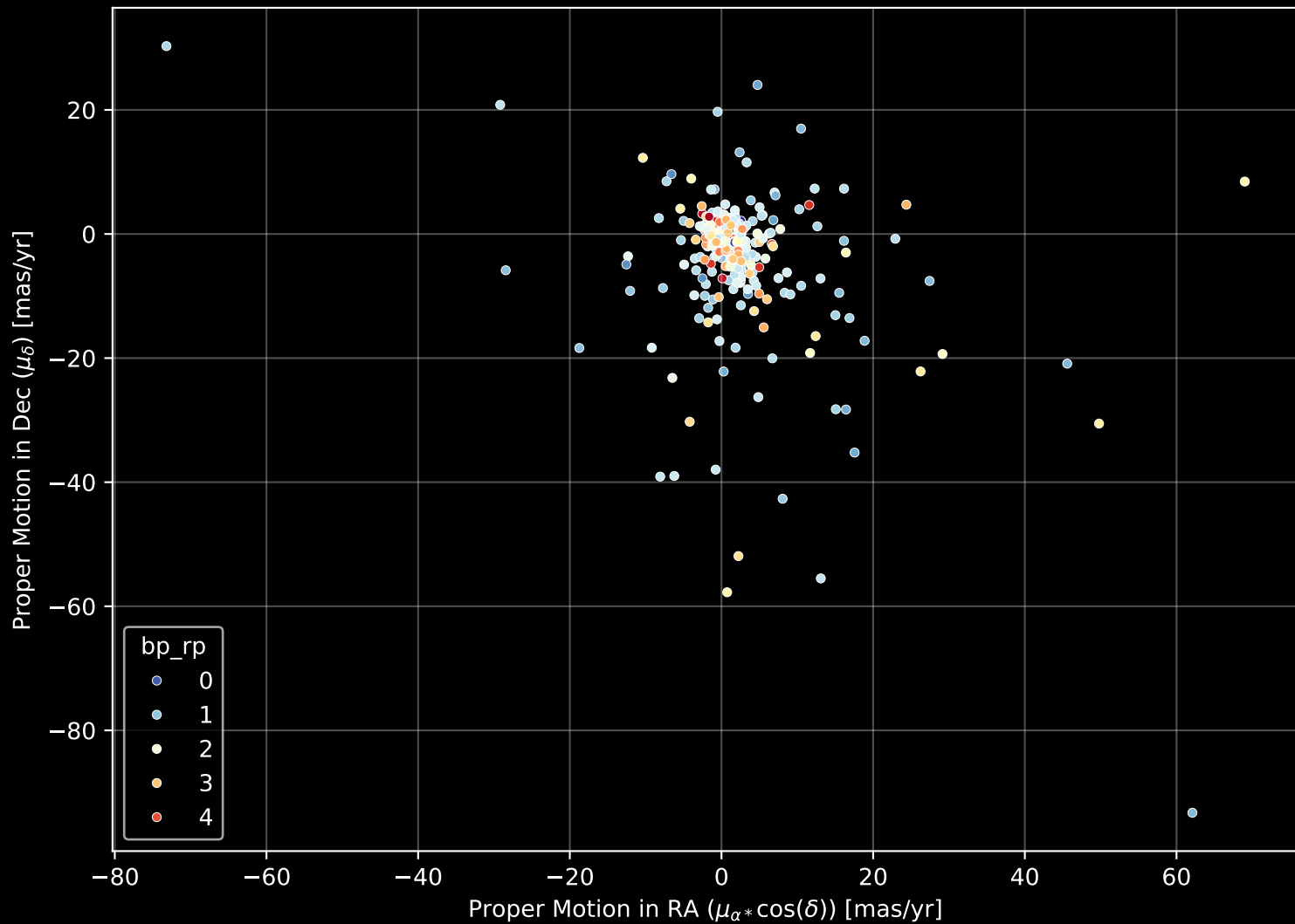
APOGEE DR17 Field: [ORIONB-B] Proper Motion Diagram (n= 384)
