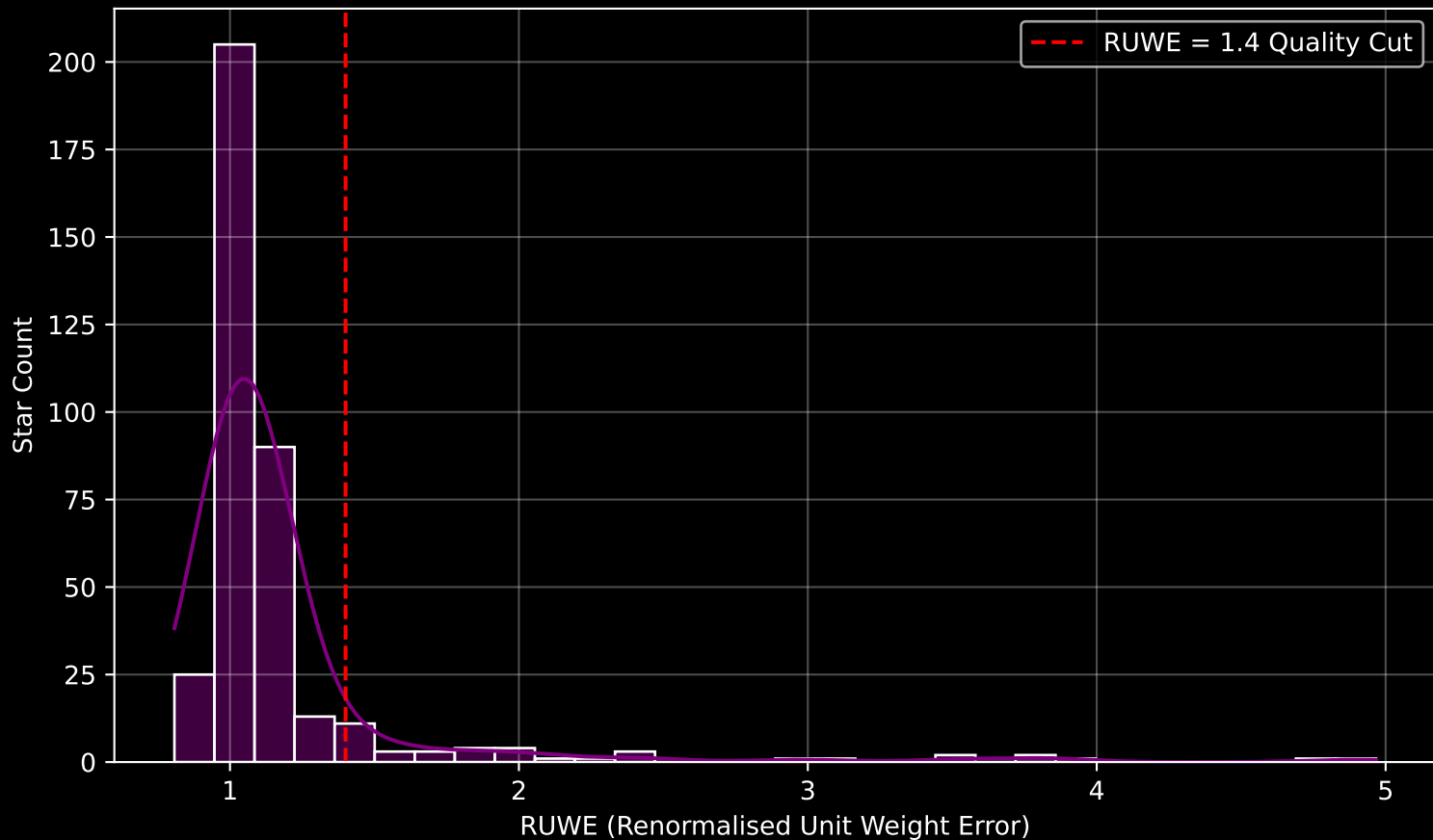
GAPOGEE DR17 Field [ORIONB-B] RUWE Distribution (n= 372)
