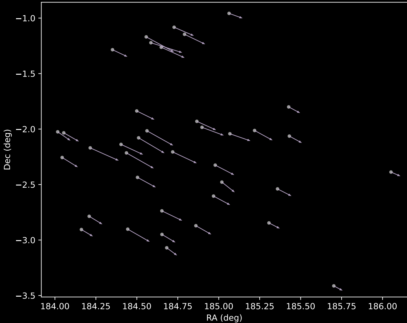
APOGEE DR17 Cluster 9 Proper Motion Vectors (n=38)
